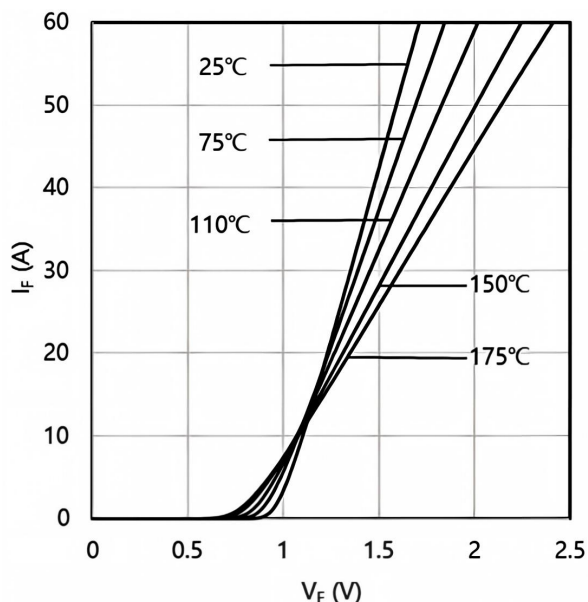
Fig.1 Forward Characteristics
