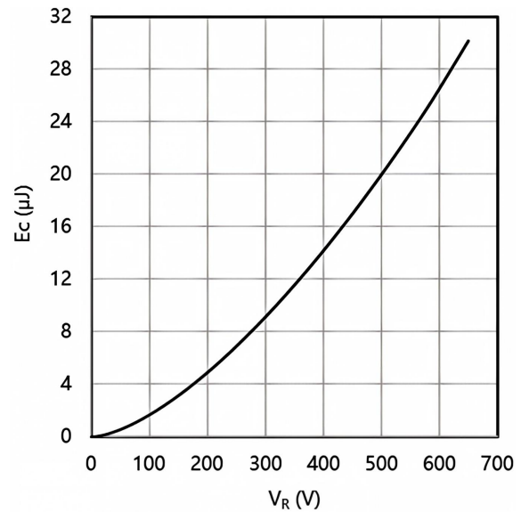
Fig.6 Capacitance Stored Energy
