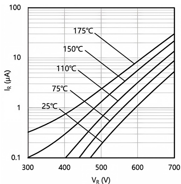
Fig.2 Reverse Characteristics
