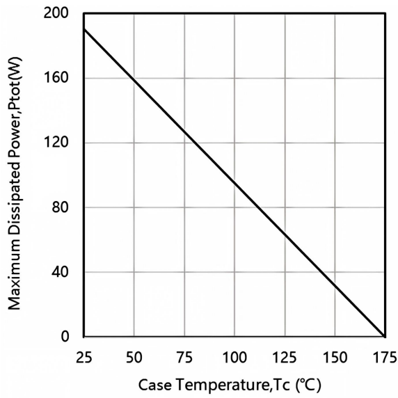
Fig.3 Power Derating
