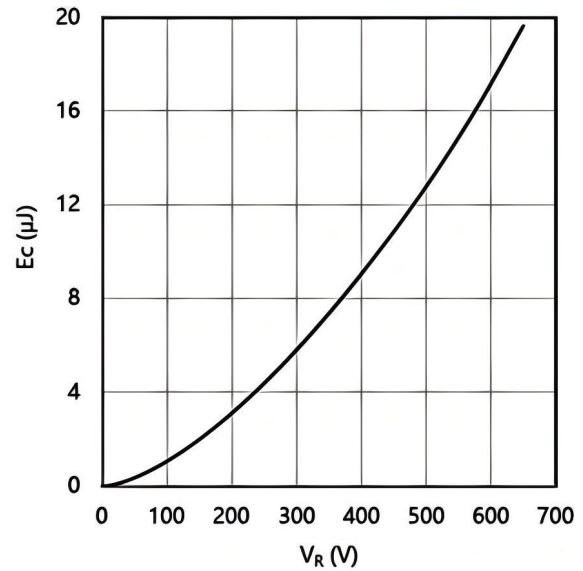
Fig.6 Capacitance Stored Energy
