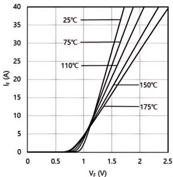
Fig.1 Forward Characteristics
