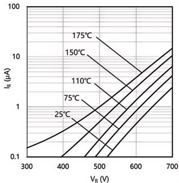
Fig.2 Reverse Characteristics
