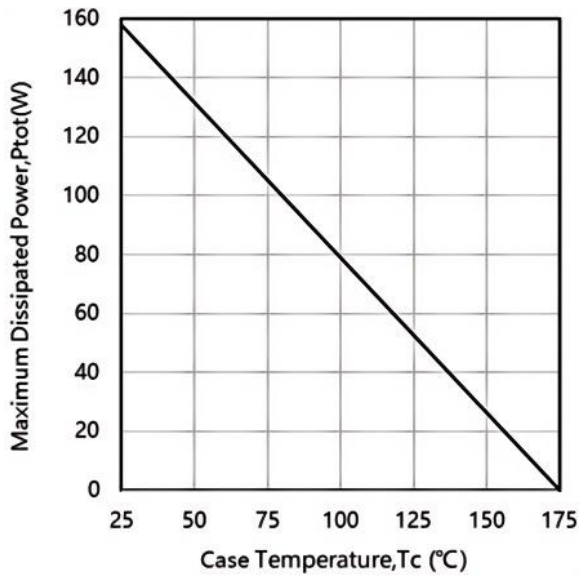
Fig.3 Power Derating
