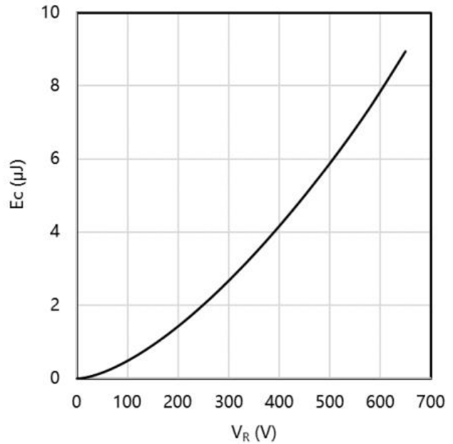
Fig.6 Capacitance Stored Energy
