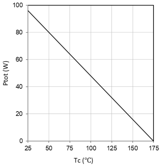
Fig.3 Power Derating
