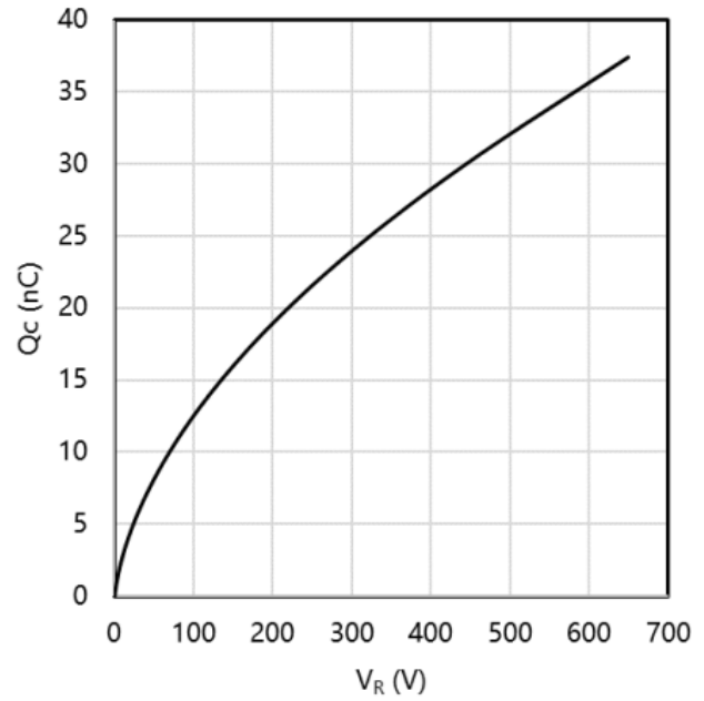
Fig.4 Total Capacitive Charge vs. Reverse Voltage
