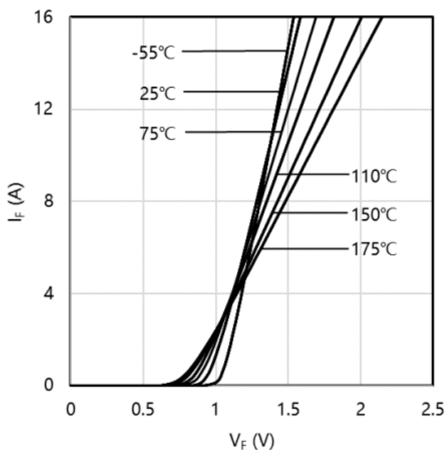
Fig.1 Forward Characteristics
