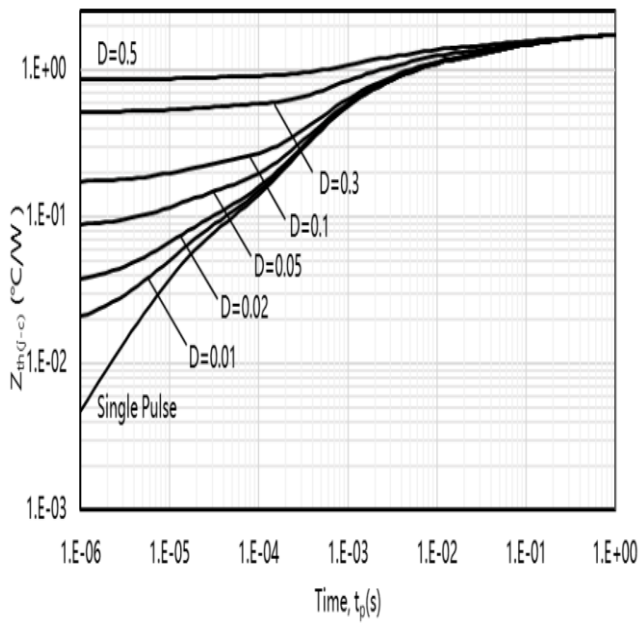
Fig.7 Transient Thermal Impedance
