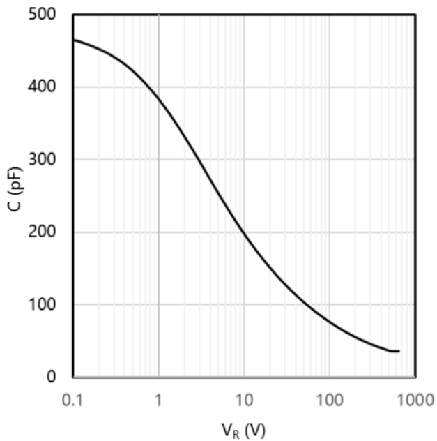
Fig.5 Total Capacitance vs. Reverse Voltage
