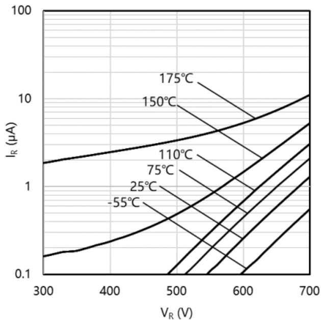
Fig.2 Reverse Characteristics
