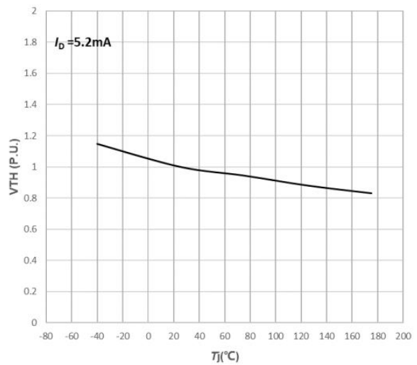
Fig6. Normalized Threshold Voltage vs. Temperature
