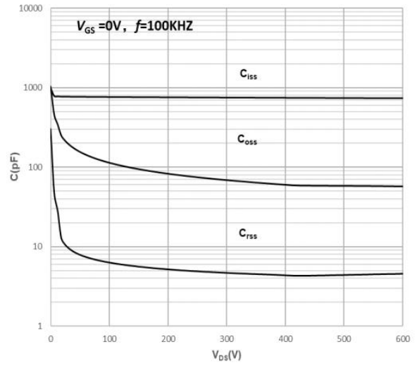
Fig8. Capacitances vs. Drain-Source Voltage (0-600V)
