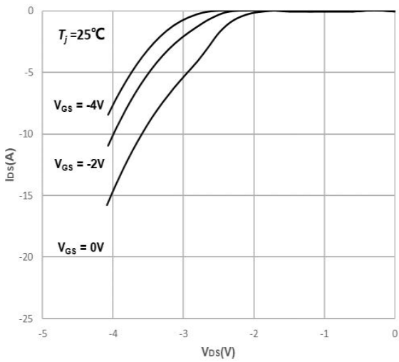
Fig9. Body Diode Characteristics
