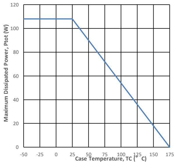
Fig12. Max Power Dissipation Derating V_{sd}
