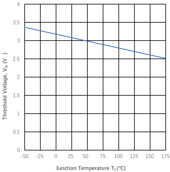
Threshold Voltage vs. Temperature
