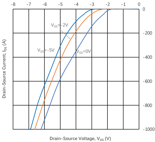
Figure 5 Body Diode Characteristic at 25°C
