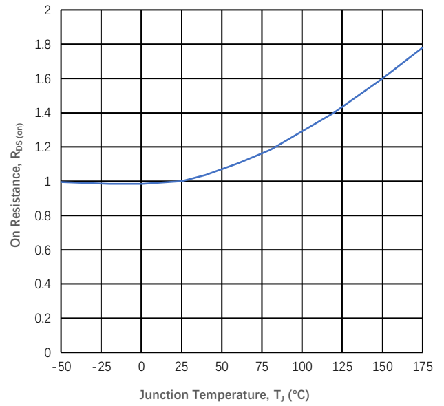
Figure 2 Normalized On-Resistance vs. T_j
