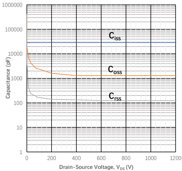
Figure 7 Typical Capacitances vs. Drain-source Voltage
