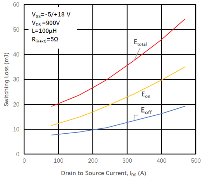
Figure 8 Inductive Switching Energy vs. Drain Current
