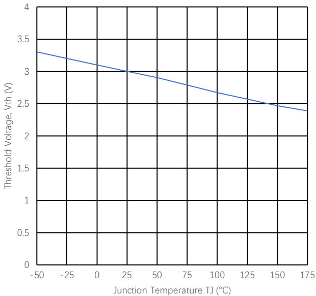
Figure 3 Threshold Voltage vs. Temperature
