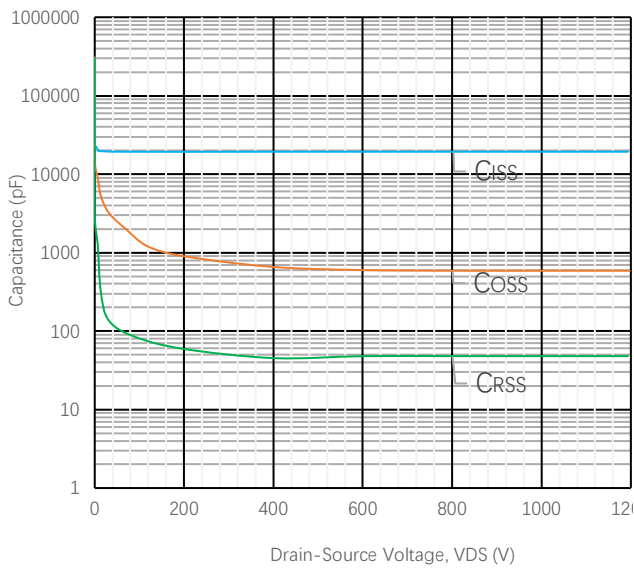
Figure 7 Typical Capacitances vs. Drain-source Voltage
