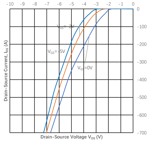
Figure 6 Body Diode Characteristic
