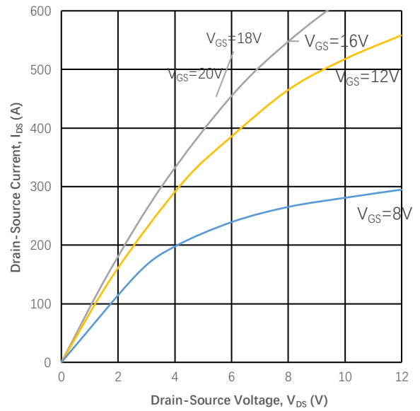
Figure 2 Typical Output Characteristics ( T_J=150\text{ }^\circ\text{C} )
