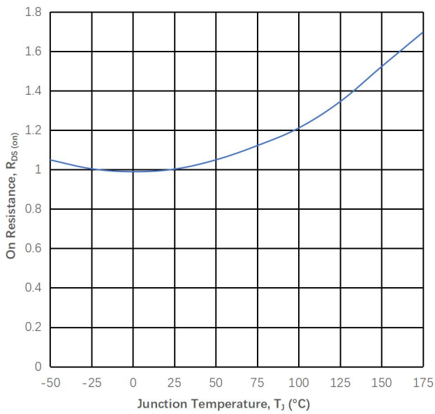
Figure 3 Normalized On-Resistance vs. Temperature
