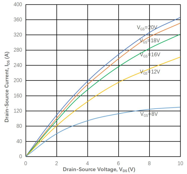
Figure 2 Output Characteristics ( T_J=175\text{ }^\circ\text{C} )
