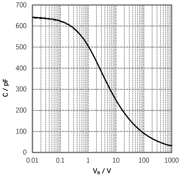
Figure 5. Capacitance vs. Reverse Voltage
