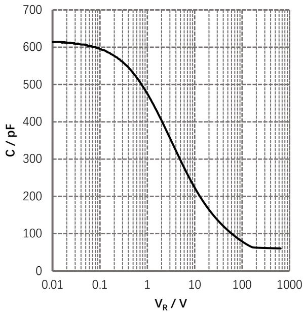
Fig 5. Typical capacitance as function of reverse voltage, C=f(V_R) ; T_j=25^\circ\text{C} ; f=1\text{ MHz}
