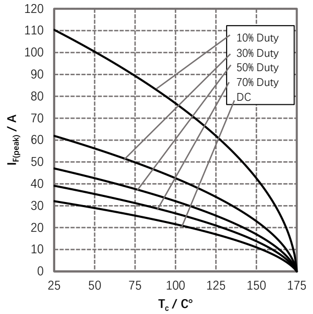
Fig 4. Current Derating
