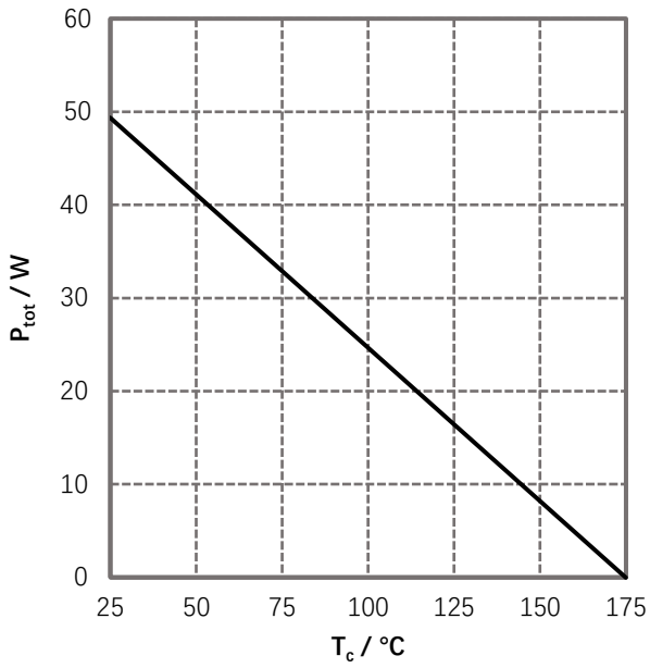
Fig 3. Power Derating
