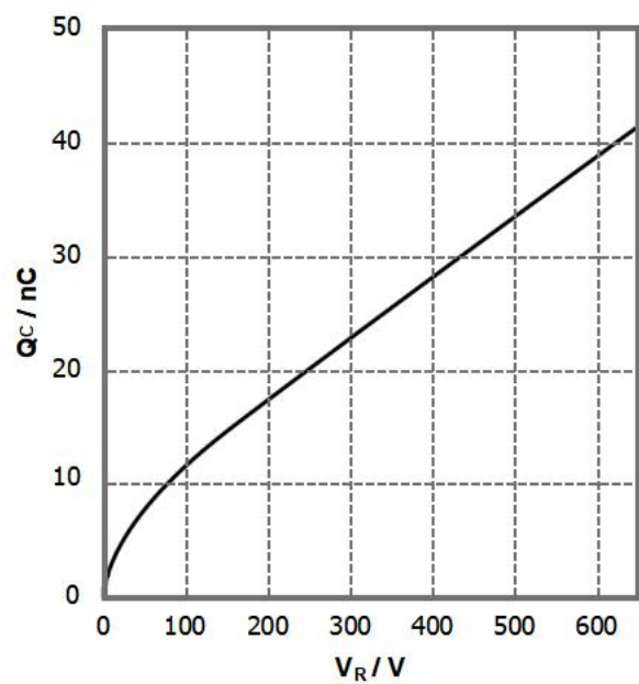
Figure 6. Reverse Charge vs. Reverse Voltage
