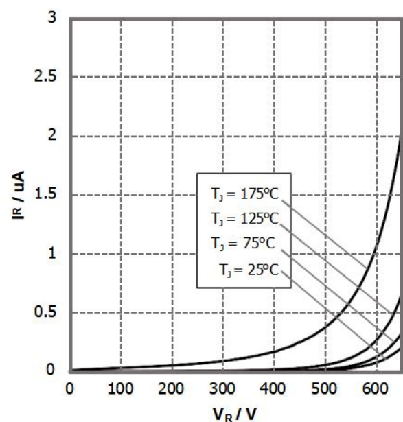
Figure 2. Reverse Characteristics
