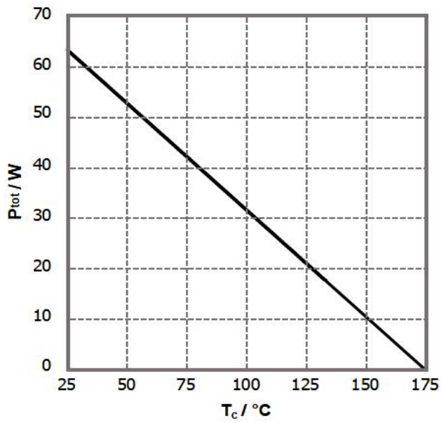
Figure 3. Power Derating
