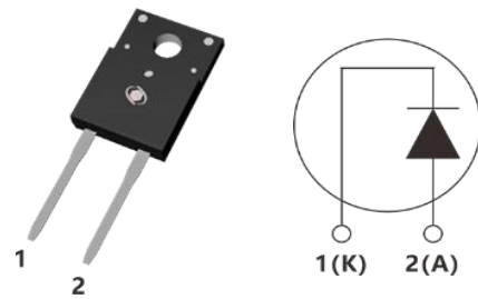
TO-220F-2L
