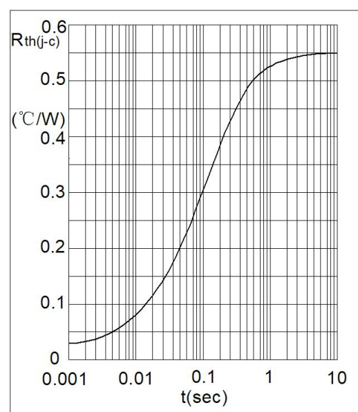
Fig4. Transient Thermal Impedance
