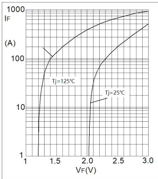
Fig1. Forward Characteristics
