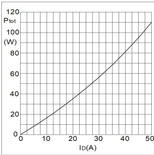
Fig1. Power Dissipation
