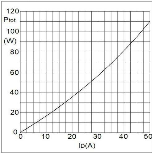
Fig1. Power Dissipation
