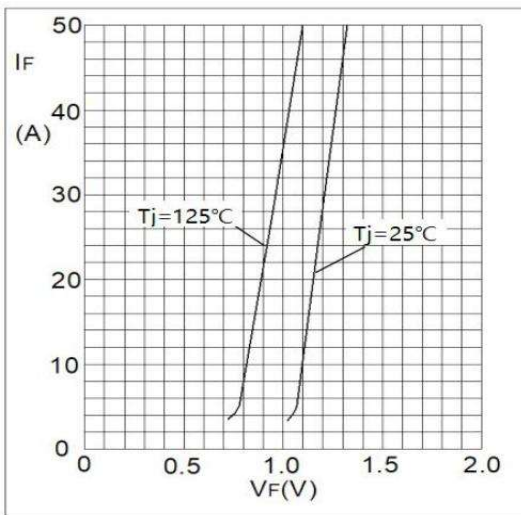
Fig3. Forward Characteristics
