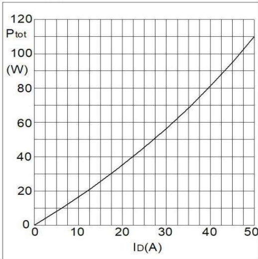
Fig1. Power Dissipation
