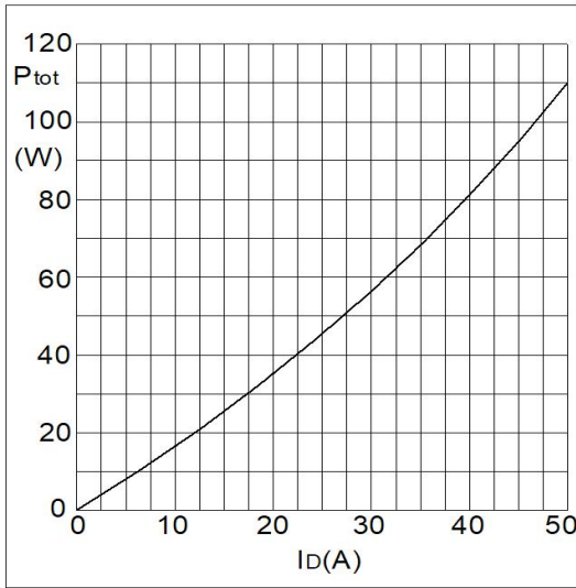
Fig1. Power Dissipation
