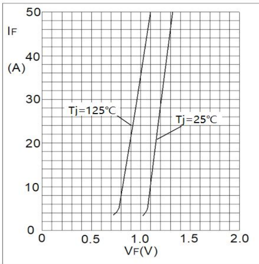
Fig3. Forward Characteristics
