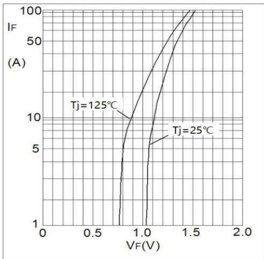
Fig3. Forward Characteristics
