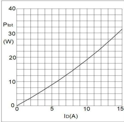
Fig1. Power Dissipation
