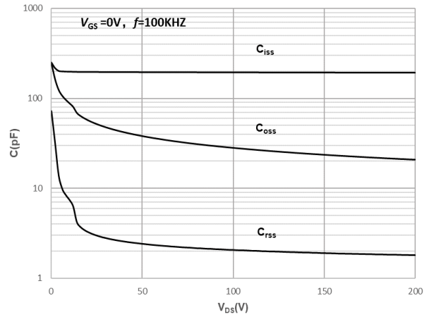
Fig7. Capacitances vs. Drain-Source Voltage (0-200V)
