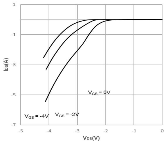
Fig9. Body Diode Characteristics T_j=25^{\circ}C
