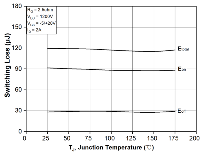
Figure 26. Clamped Inductive Switching Energy vs. Temperature
