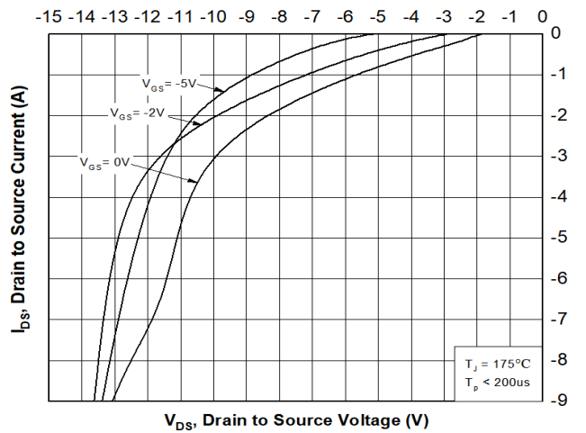
Figure 10. Body Diode Characteristic at T_J = 175\text{ }^{\circ}\text{C}
