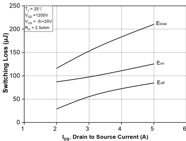
Figure 23. Clamped Inductive Switching Energy vs. Drain Current ( V_{DD} = 1200V )
