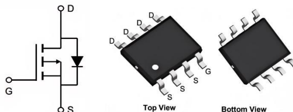
SOP-8
